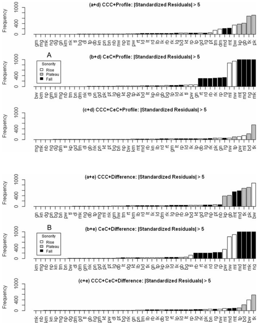
Fig. 2 Ranked frequencies with which the absolute value of the standardized residual for a cluster exceeded 5, from 1000 iterations of the (panel A, a–c+d) Profile, (panel B, a–c+e) Difference, and (panel C, a–c+g) interaction of Values models. White bars represent clusters in which sonority rises, gray bars those in which it plateaus, and black bars those in which it falls
