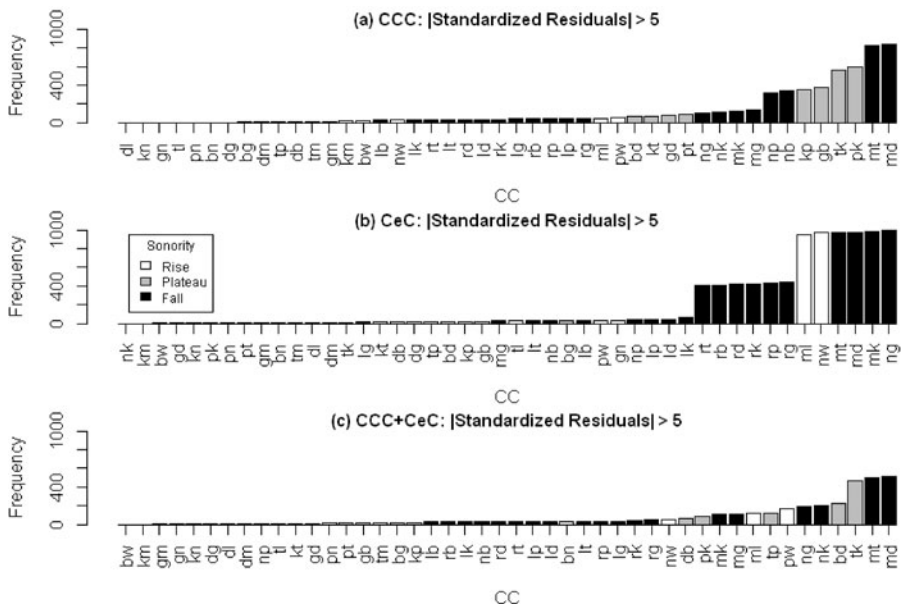
Fig. 1 Ranked frequencies with which the absolute value of the standardized residual for a cluster exceeded 5, from 1000 iterations of the (a) CCC, (b) CeC, and (c) CCC+CeC models. White bars represent clusters in which sonority rises, gray bars those in which it plateaus, and black bars those in which it falls
