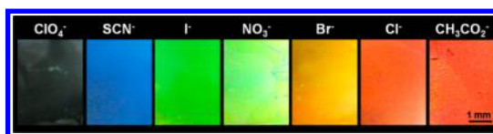
Figure 2. Color change of the photonic gel films quaternized for 36 h with direct exchange of counteranions. The color of the photonic gel films shifts from transparent to blue, green, and red with increasing hydration energy of the counteranions. The photographs were taken on a black background under fluorescent lights, and the counterions were exchanged using 10 mM solution of a variety of tetrabutylammonium salts.
